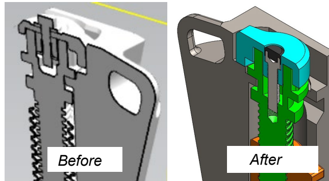
Fig 6. Parts of the new wedge
