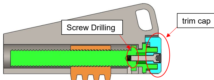
Fig 7. Power wedge side view
