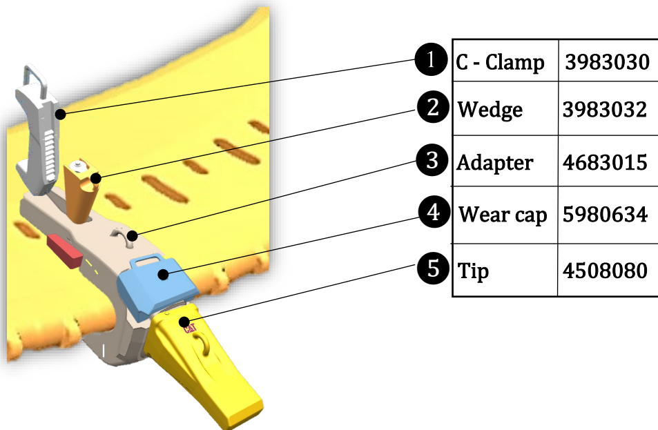
Fig 2. System Parts
